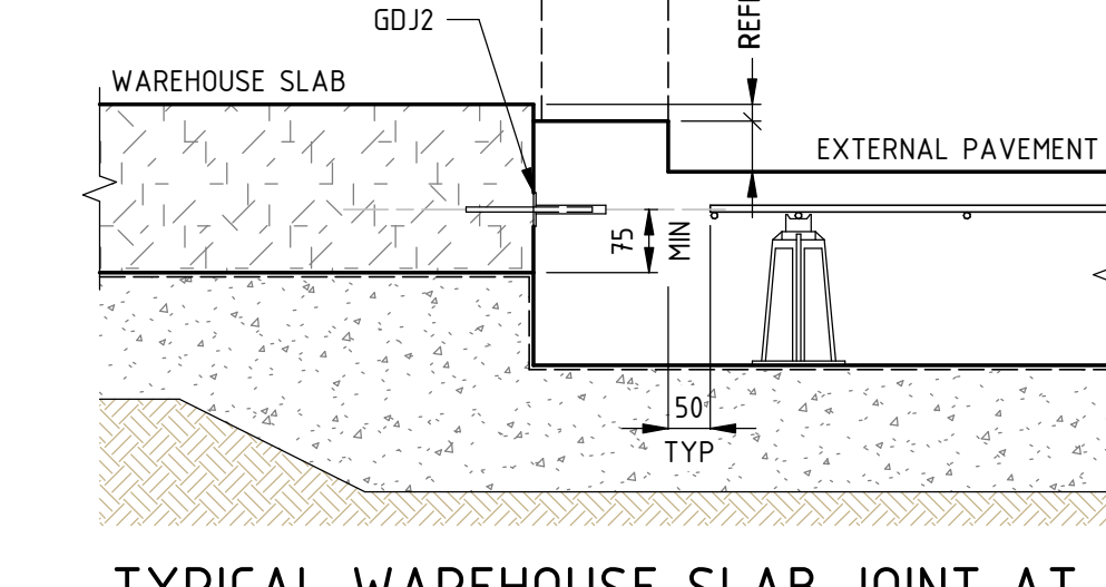
TYPICAL WAREHOUSE SLAB JOINT AT PEDESTRIAN DOOR DETAIL
