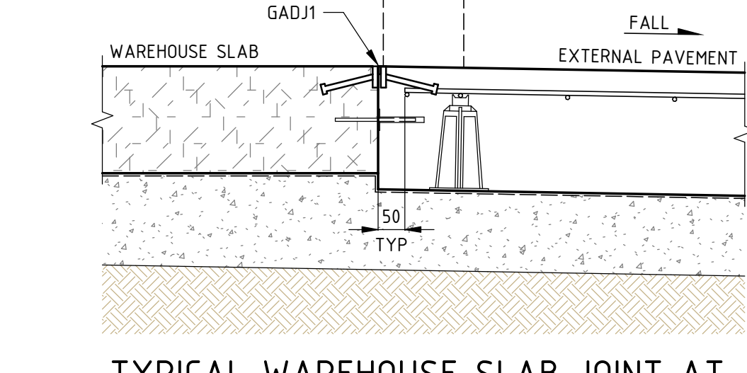
TYPICAL WAREHOUSE SLAB JOINT AT ROLLER DOOR DETAIL
