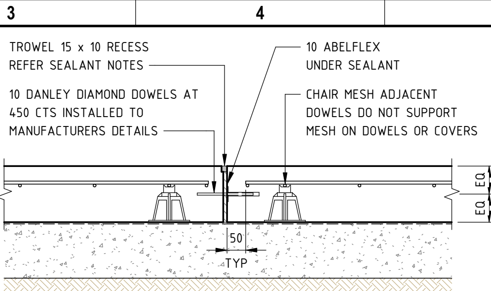
TYPICAL DOWEL JOINT 1 DETAIL (DJ1)
