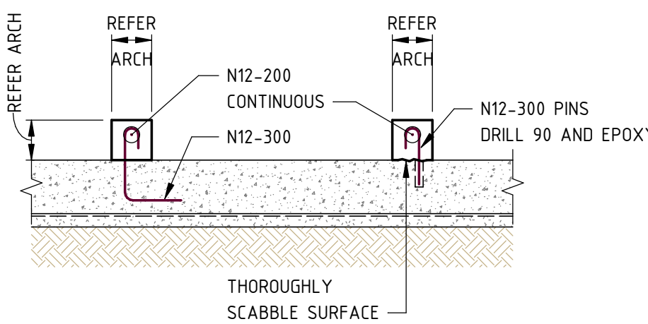
TYPICAL HOB UNDER 190 WIDE DETAIL
