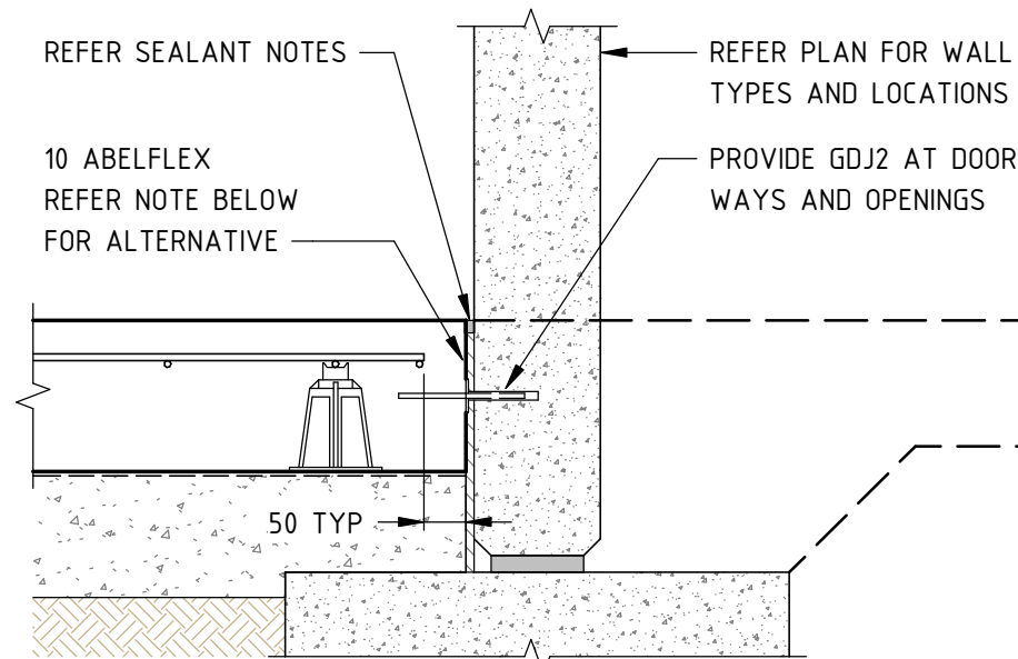
TYPICAL ISOLATION JOINT DETAIL (ISJ)
