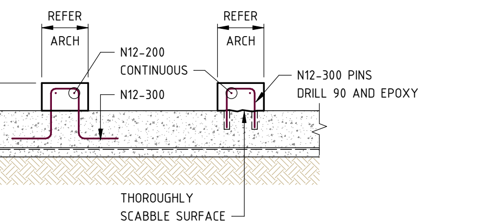
TYPICAL HOB OVER 191 WIDE DETAIL
