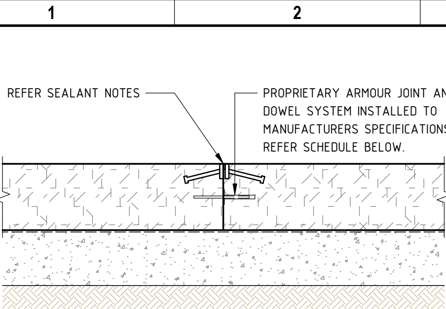
TYPICAL ARMoured DOWEL JOINT (ADJ1)
