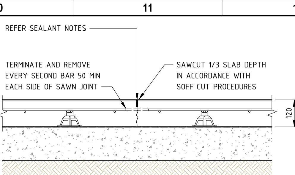
TYPICAL SAWN JOINT 2 DETAIL (SJ2)
