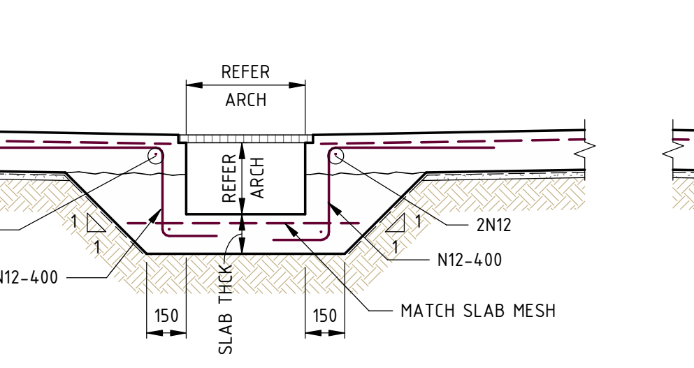
TYPICAL GRATED DRAIN DETAIL
