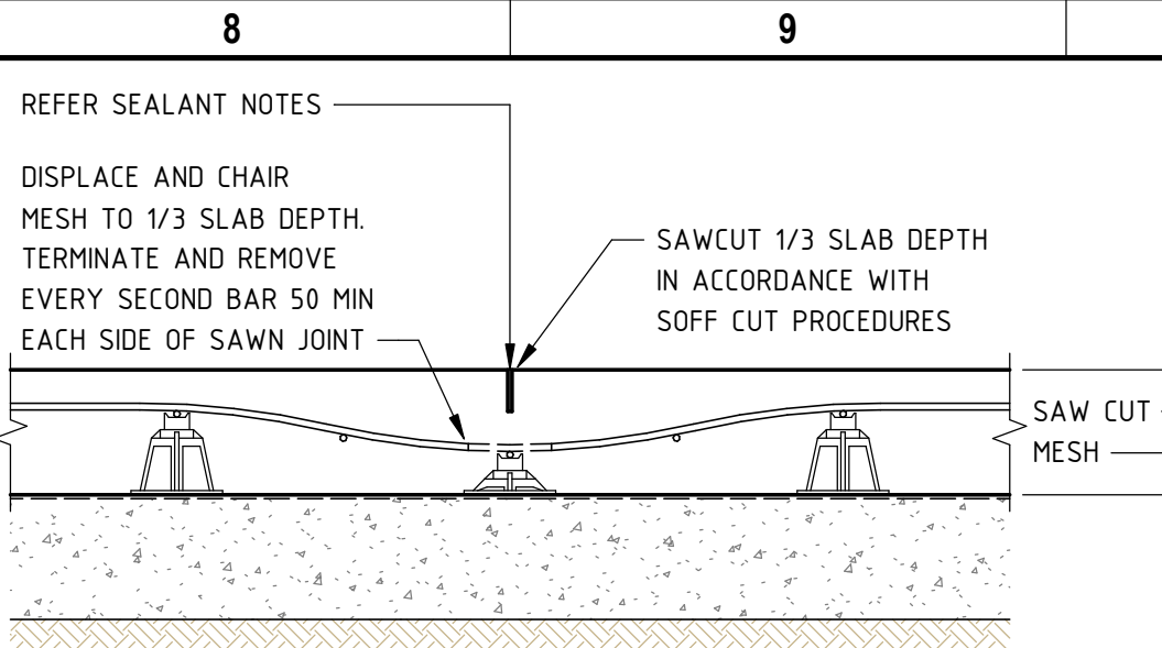
TYPICAL SAWN JOINT 1 DETAIL (SJ1)
