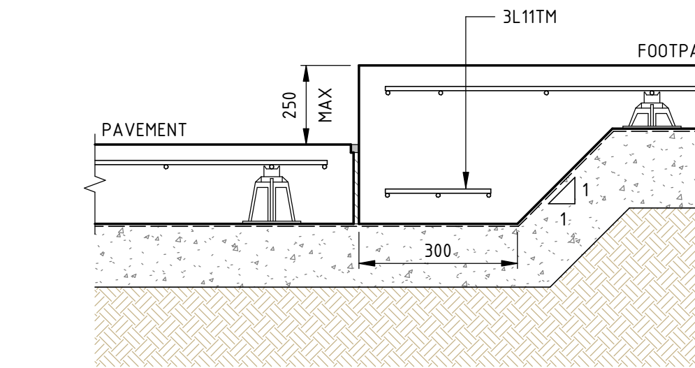
TYPICAL EXTERNAL PAVEMENT KERB STEP TO FOOTPATH SLAB DETAIL
