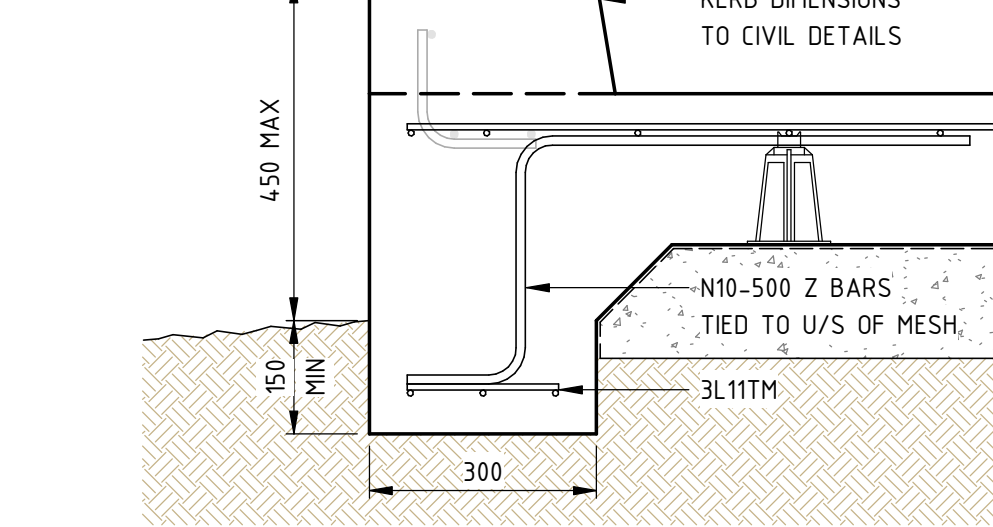
TYPICAL EXTERNAL PAVEMENT KERB AND TURNDOWN DETAIL AT BOUNDARY
