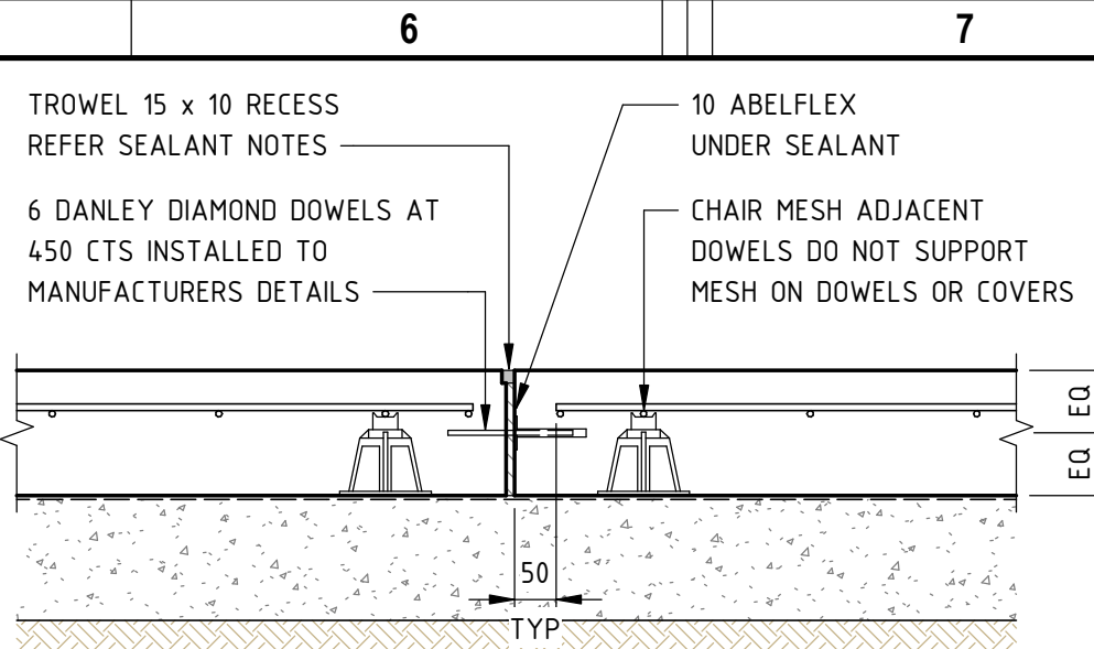
TYPICAL DOWEL JOINT 1 DETAIL (DJ2)
